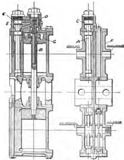
FIG. 200.—Sectional View of the Valve Motion and Mechanism of the "Victor" Auxiliary Steam Pumps.
